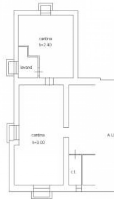
PIANO INTERRATO
